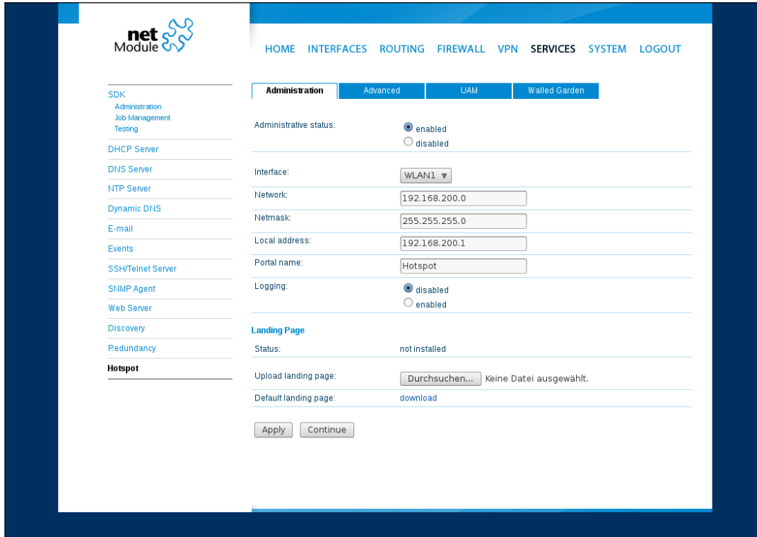
Figure 5.5: HotSpot Configuration
